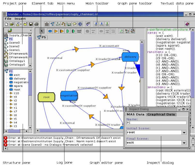
Figure 4. Islander Graphical Editor for E-Institutions
