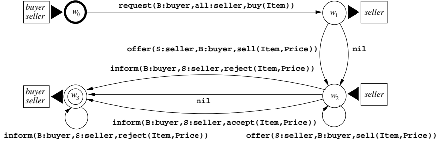
Figure 2. Simple Agora Room Scene
