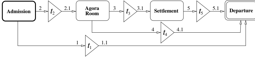
Figure 3. E-Institution for Simple Agoric Market
