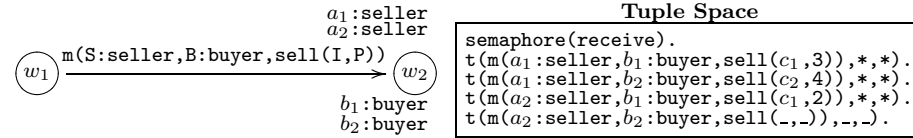
Figure 22. Enactment of Agora Room Scene (receive Stage)
