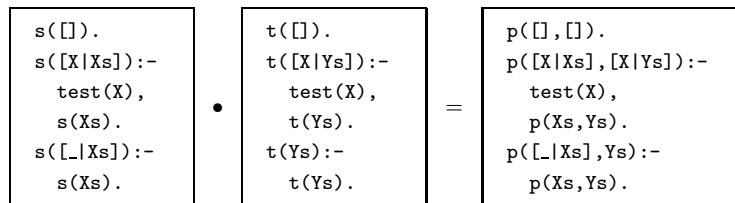
Figure 11. Skeleton • Technique = Program
