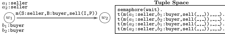
Figure 20. Enactment of Agora Room Scene ( wait Stage)
