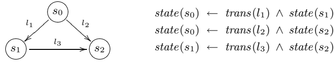
Figure 8. State Transitions and Horn Clauses
