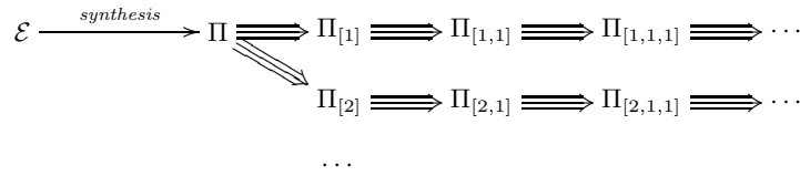
Figure 14. Exploring and Organising a Design Space
