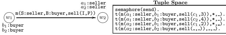
Figure 21. Enactment of Agora Room Scene (send Stage)
